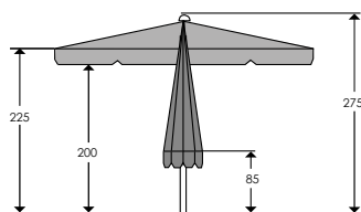
Dimensions (cm) for size 300 cm Ø:
