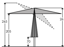
Dimensions (cm) for size 300 x 200 cm:
