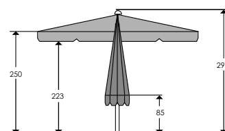
Dimensions (cm) for size 300 x 300 cm:
