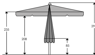
Dimensions (cm) for size 400 cm Ø:
